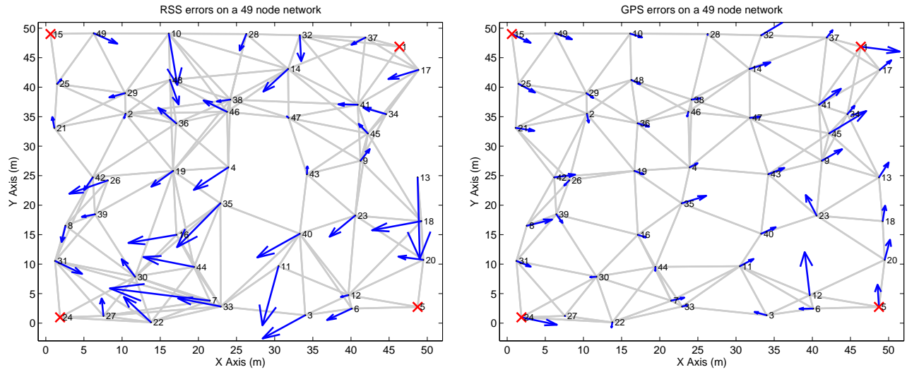
Figure 8: 49 Node network "X"'s indicate anchor nodes, dots are mobile nodes, and arrows indicate localization errors. Edges in the left graph indicate radio connectivity, in the right graph they indicate distances of 15m or less. RSS localization (left) is coping with a connectivity hole in the center of the network. GPS localization (right) does quite well.
